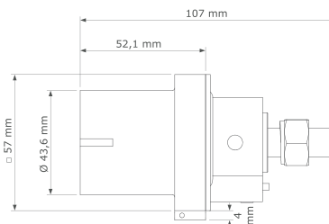
Panel source with M12 threaded post
