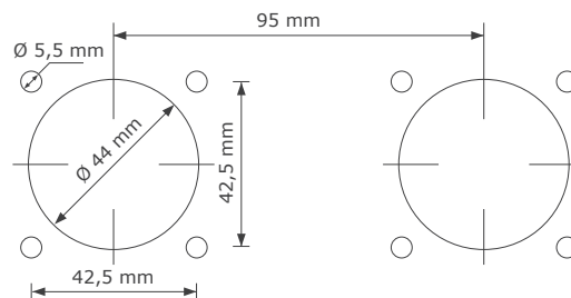
Basic panel source front mounted
