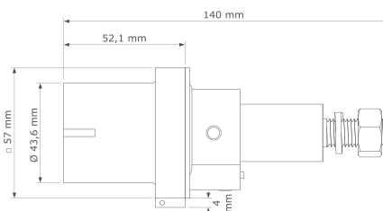
Panel source Extended length contact with M12 threaded post
