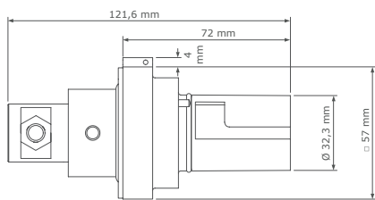
Basic panel drain with EasiLug
