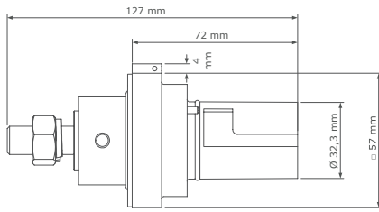
Basic panel drain with M12 threaded post
