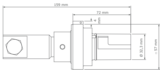
Basic panel drain with ComLug L2
