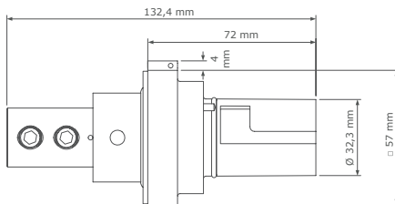
Basic panel drain with set screw contact
