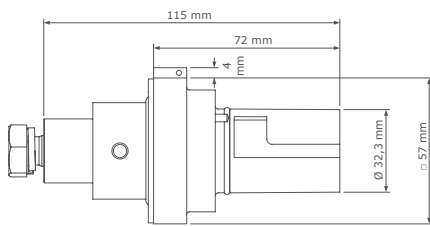
Basic panel drain with M12 threaded hole
