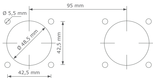
Basic panel drain rear mounted
