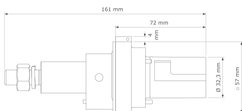
Panel drain with M12 threaded hole
