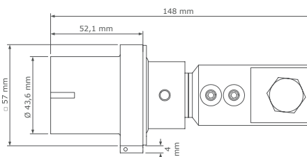
Basic panel source with ComLug L2
