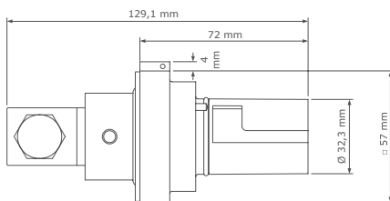
Basic panel drain with ComLug L
