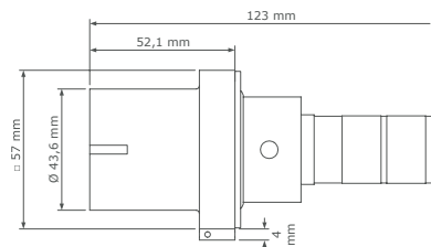
Basic panel source with crimp contact
