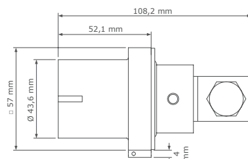
Basic panel source with ComLug L
