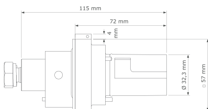
Panel drain with M12 threaded hole
