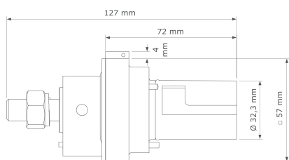
Panel drain with M12 threaded post
