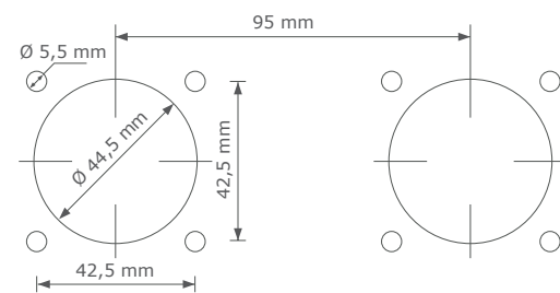
Basic panel source rear mounted
