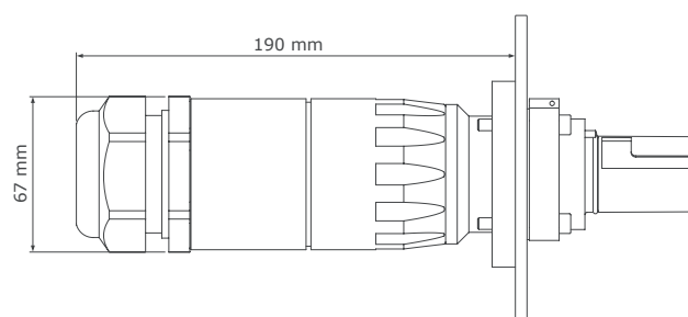
Long version with M50 gland
