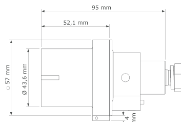
Panel source with M12 threaded hole
