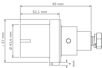
Basic panel source with M12 threaded hole
