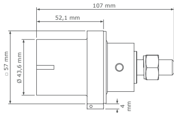
Basic panel source with M12 threaded post
