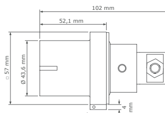
Basic panel source with EasiLug
