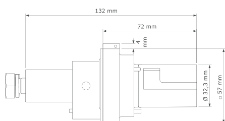
Panel drain Extended length contact with M12 threaded hole
