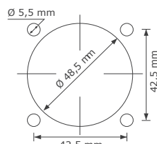
Panel drain front/rear
