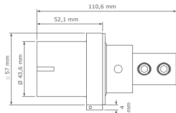
Basic panel source with set screw contact
