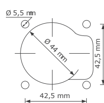
Panel source front/rear
