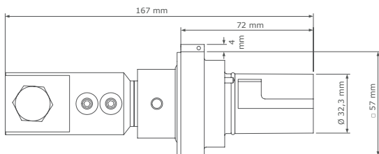
Basic panel drain with ComLug XL
