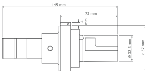
Basic panel drain with crimp contact
