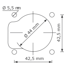
Panel drain front/rear
