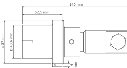
Basic panel source with ComLug L2
