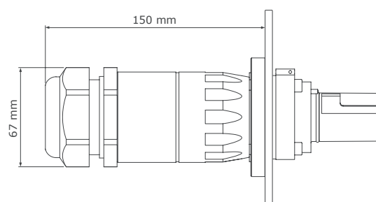
Medium version with M50 gland
