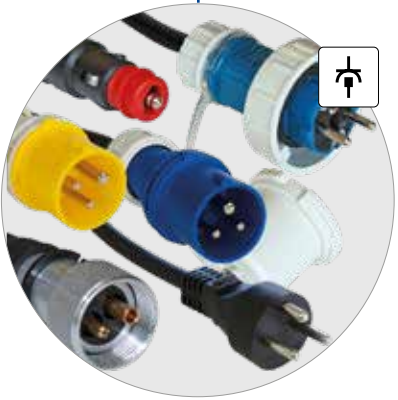
Power cable can be removed/swapped Alternative plug systems and power cable lengths on request
