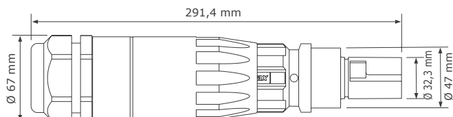
Oversized body
