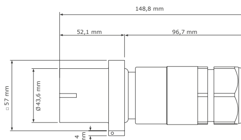
Shelter panel source with standard backshell
