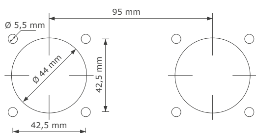
Panel drain front/rear
