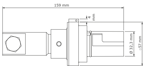
Basic panel drain with ComLug L2
