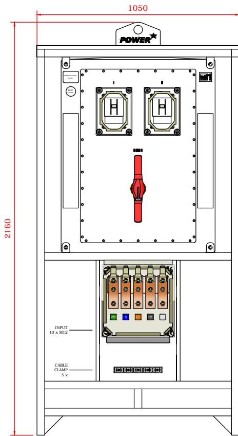
FRONT
